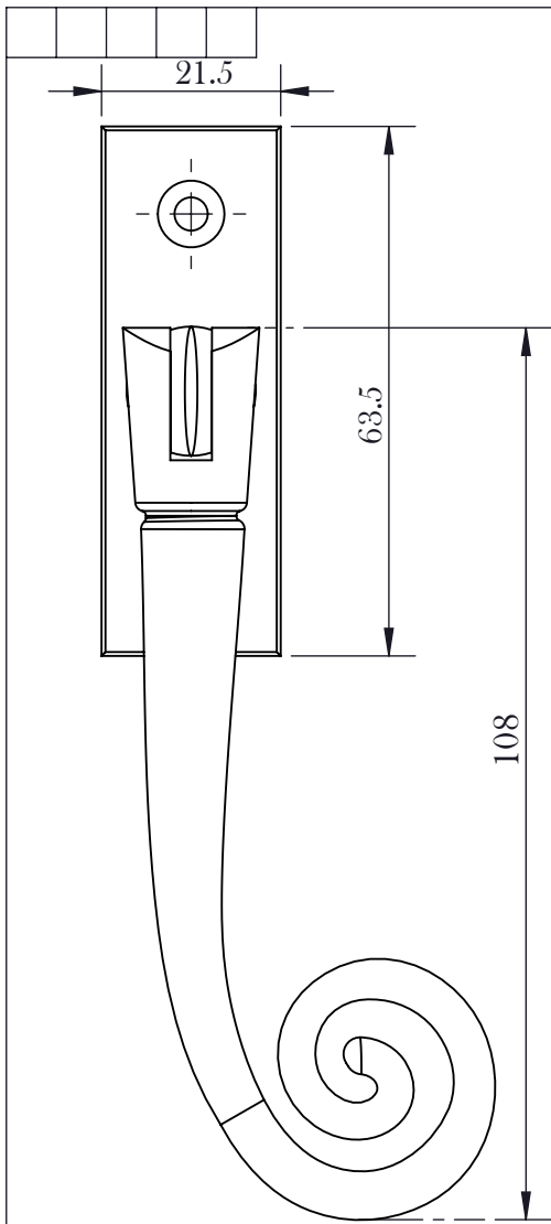
TOP VIEW
