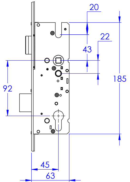
DETAIL A SCALE 1 : 3
