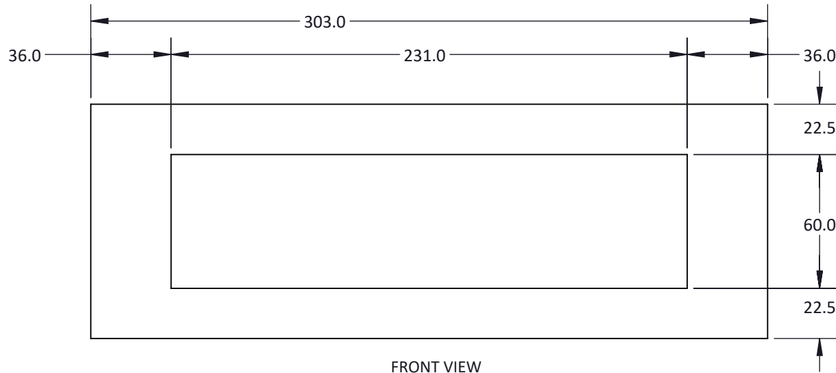
FRONT VIEW
