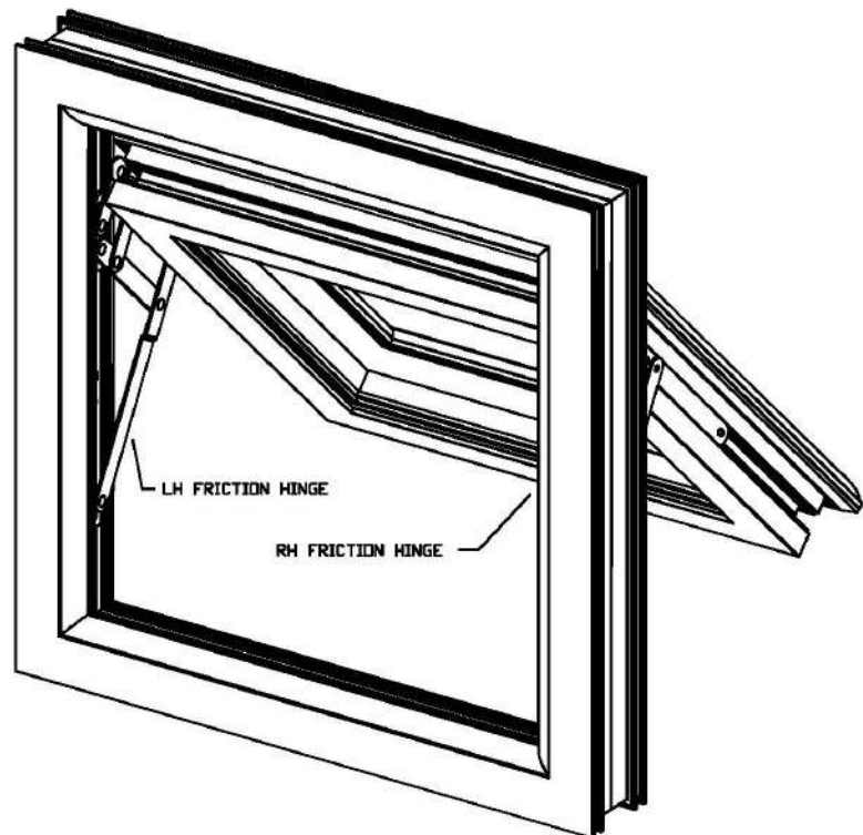
TOP HUNG SASH
