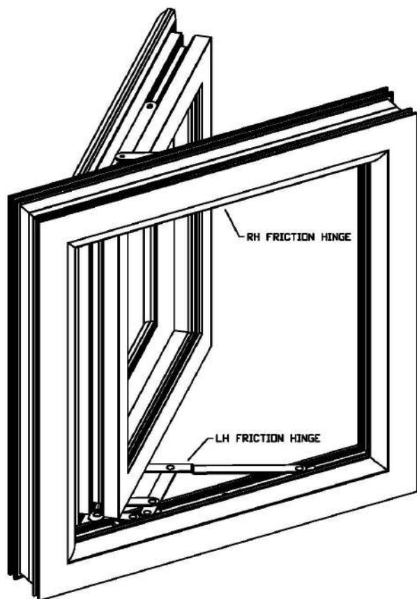
SIDE HUNG SASH
